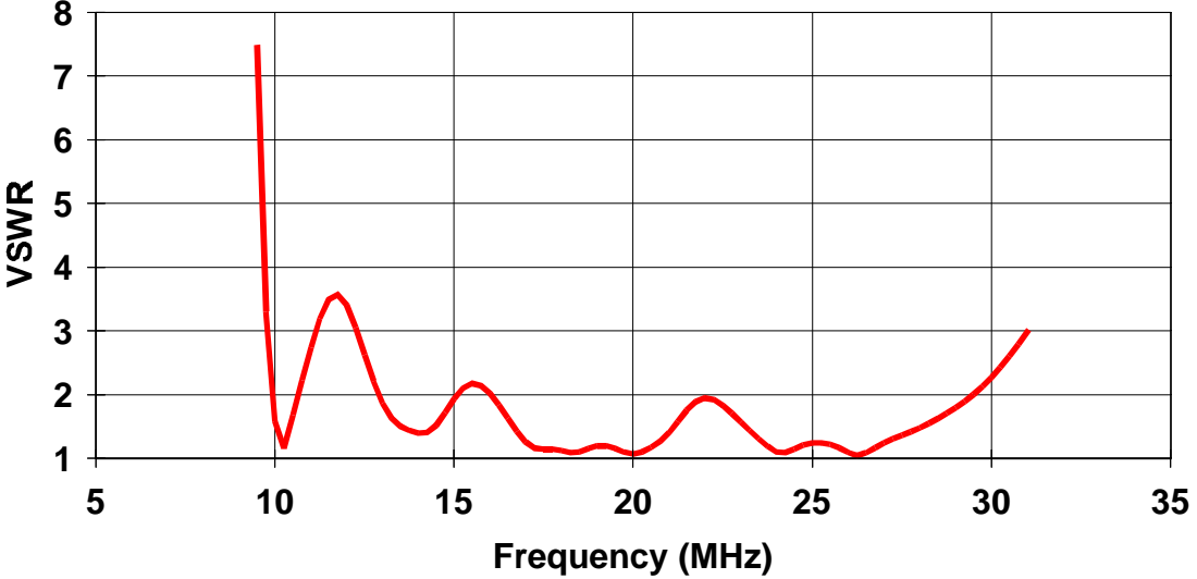
VSWR vs Frequency
